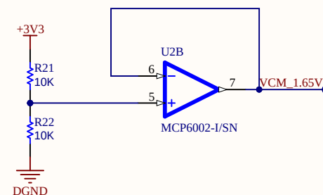
Offset 1.65V
